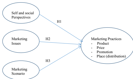
Figure 1. Theoretical Framework
