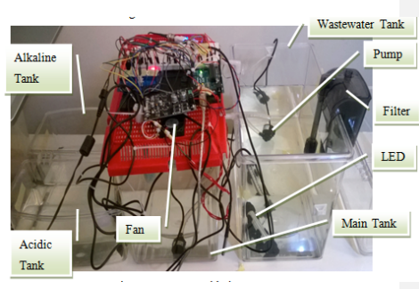
Figure 2.0. Hardware components interfaced with LabVIEW Figure 2.1. Low cost prototype
