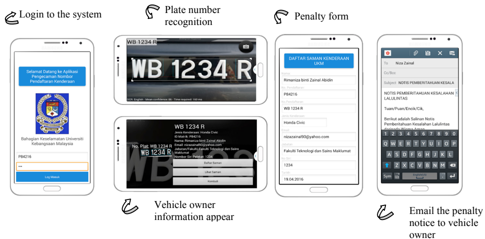
Figure 3. Application Interface
