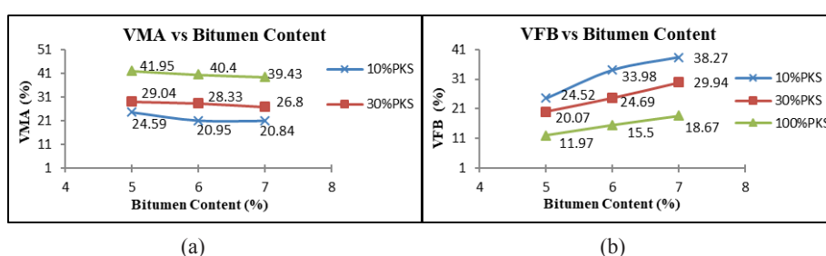
Figure 7. (a) Voids in Minerals Aggregates percent curves for modified; and (b) Voids Filled with Bitumen percent curves for modified mixes
