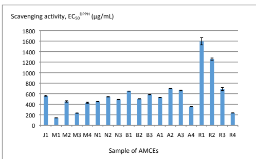
Figure 5. DPPH-free radical scavenging activity of 19 samples of Annona muricata crude extract. The scavenging activities of the AMCE samples were evaluated as the \text{EC}_{50}^{\text{DPPH}} , the concentration of antioxidants that reduces the DPPH-free radical by about 50%. Each value is expressed as the mean from the three replicates and the error bars indicate standard deviations
