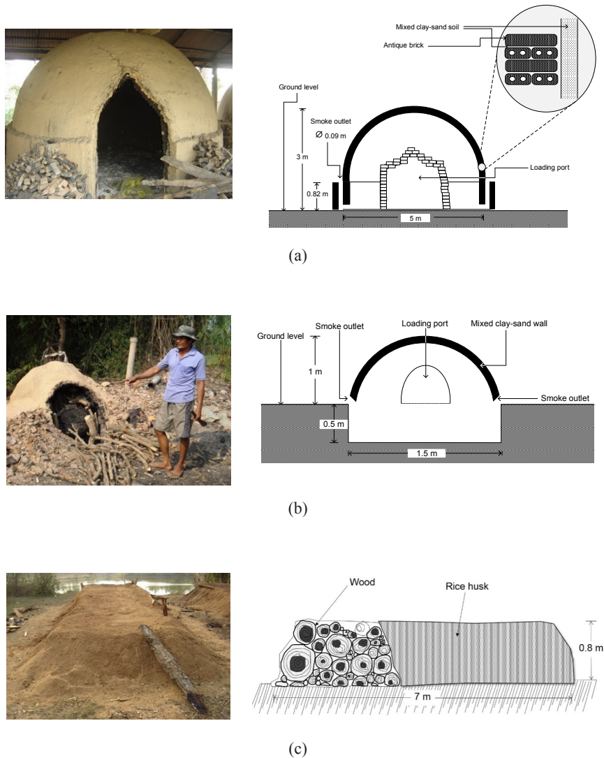
Figure 2. Kiln types and their construction used for charcoal production in Northeast Thailand: (a) high capital and permanent kiln; (b) low capital and permanent kiln; and (c) low capital and temporary kiln
