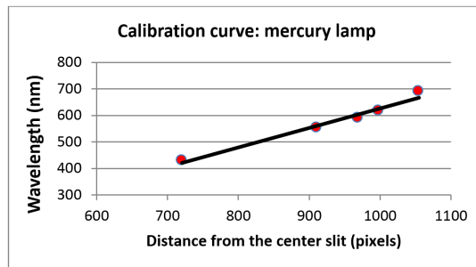
Figure 6. Calibrating a home-made spectrometer using a mercury lamp with known spectra. The top panel shows the tracker window where the calibration involves two processes: 1) setting up the coordinate system and 2) placing calibration points at spectral lines with known wavelength. The calibration points mark the distance (measured in pixels) from the reference point, which is taken as bright white line at the right. The bottom panel shows the calibration curve for the mercury lamp which is done by correlating the distance from the reference point with the known wavelength.
