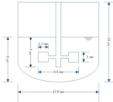
Fig.3: Geometry of the bioreactor.
